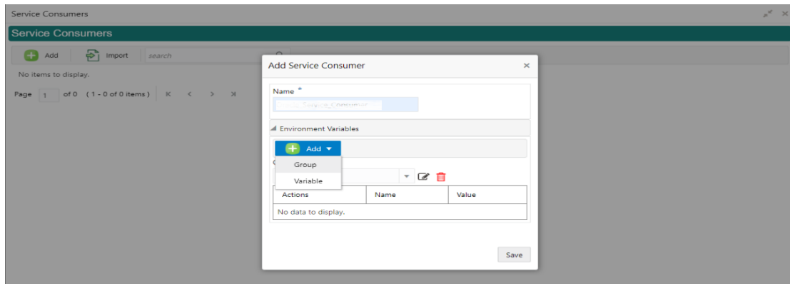
Figure 118: Environment Variables
