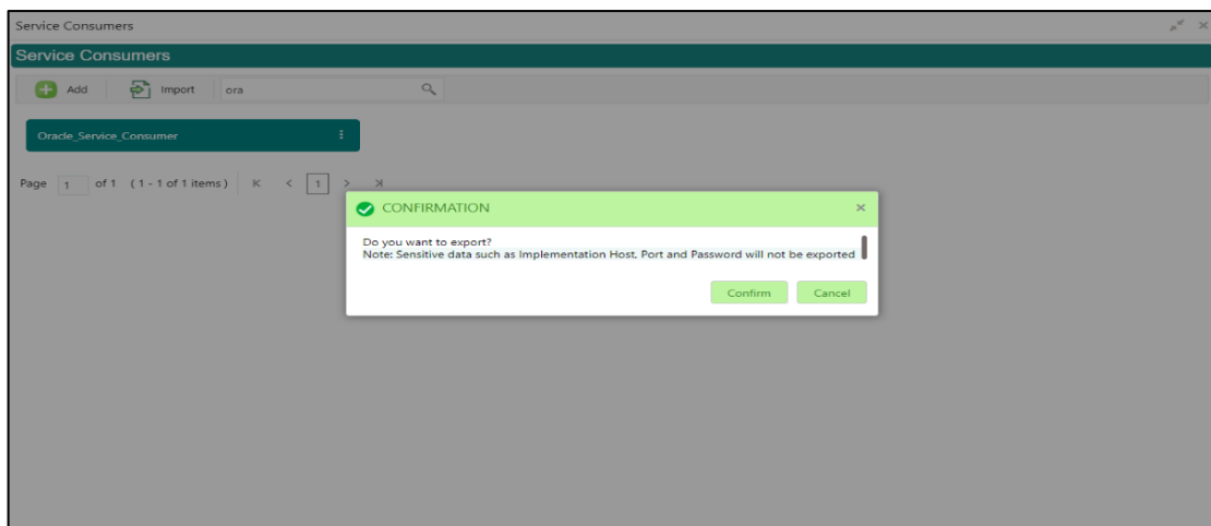
Figure 77: SQL Export
