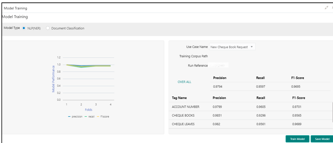
Figure 245: Model Training
