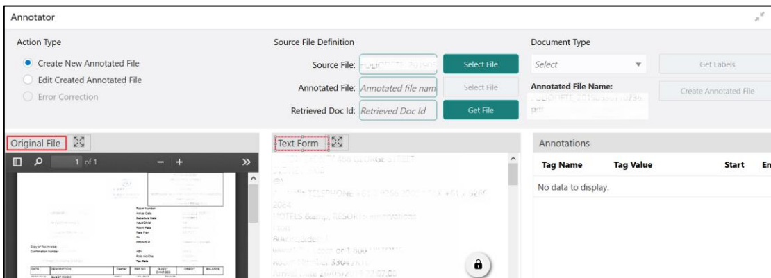
Figure 238: Text Form
