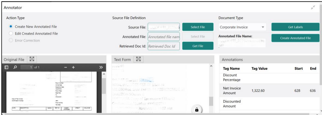
Figure 243: Annotations
