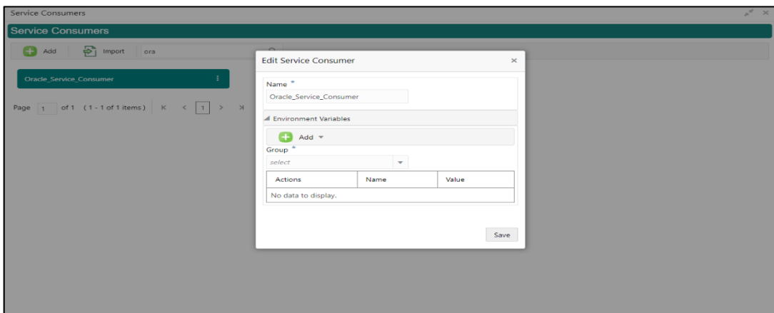
Figure 74: Edit
