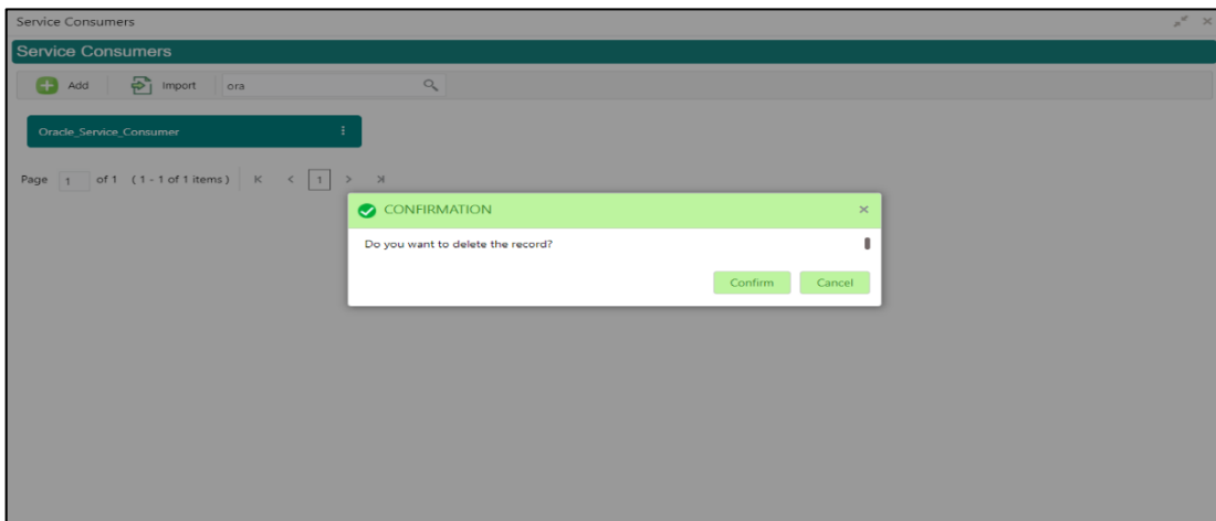
Figure 123: Delete
