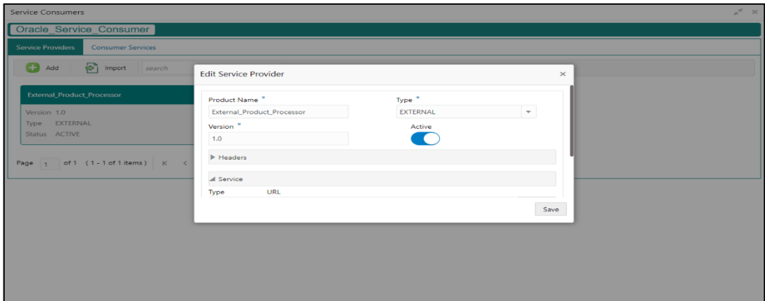
Figure 86: Edit
