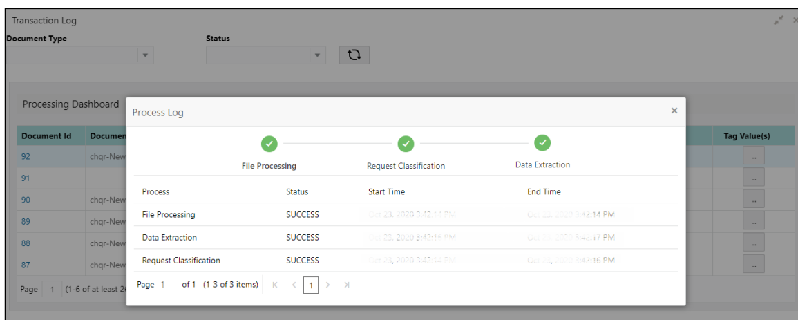
Figure 251: Execution Flow
