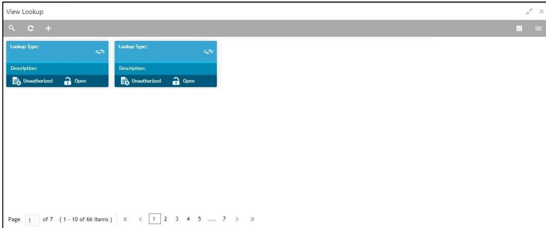
Figure 100 : View Lookup
