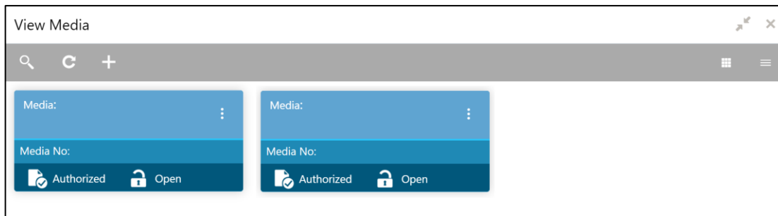
Figure 51: View Media
