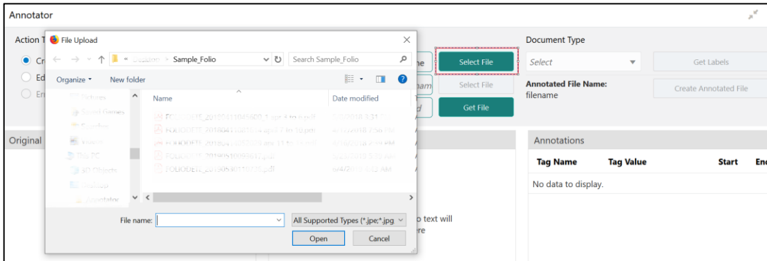
Figure 237: File Upload
