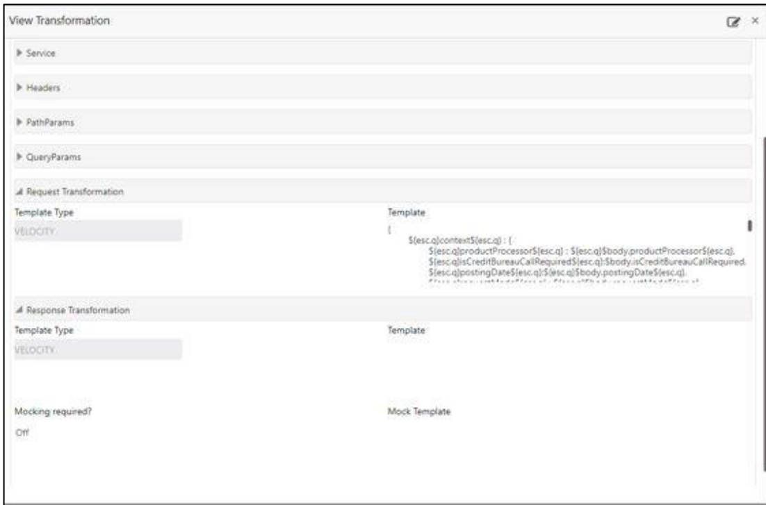
Figure 139: Consumer Services
