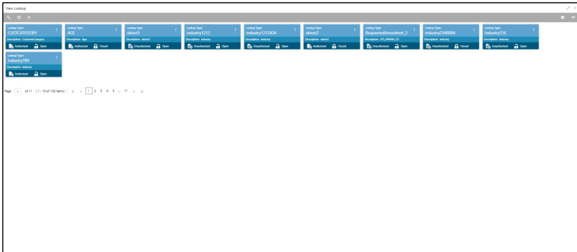
Figure 148 : View Lookup
