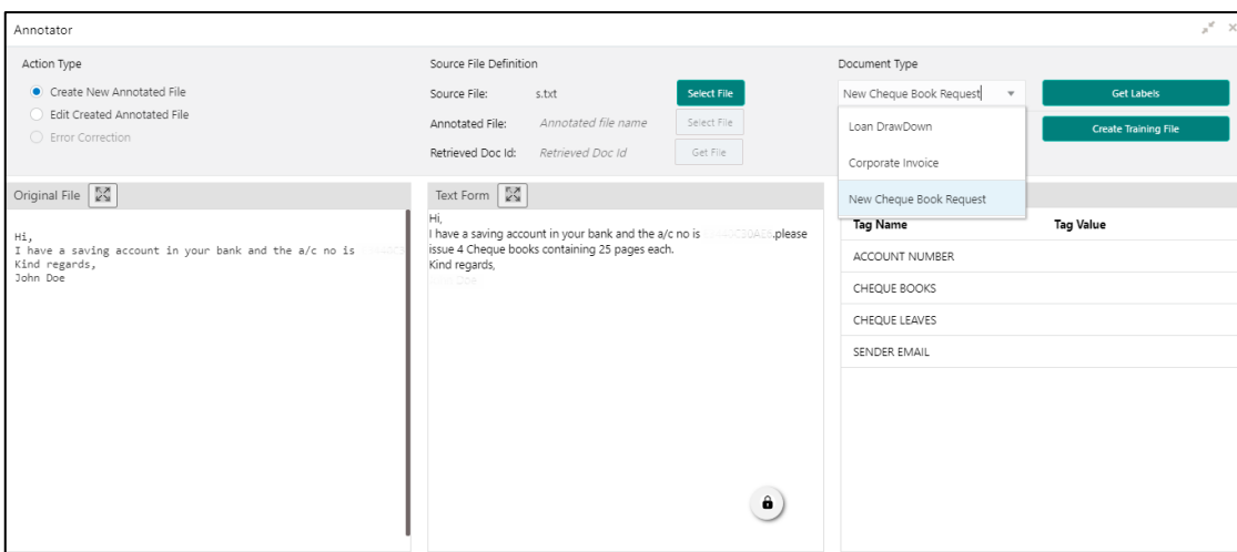
Figure 235: Annotator
