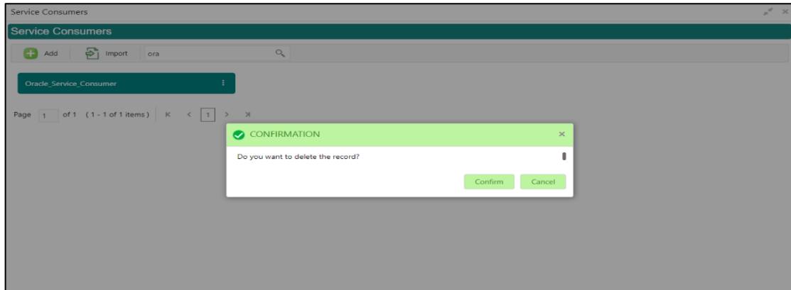
Figure 75: Delete
