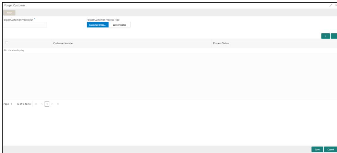
Figure 44: Forget Customer
