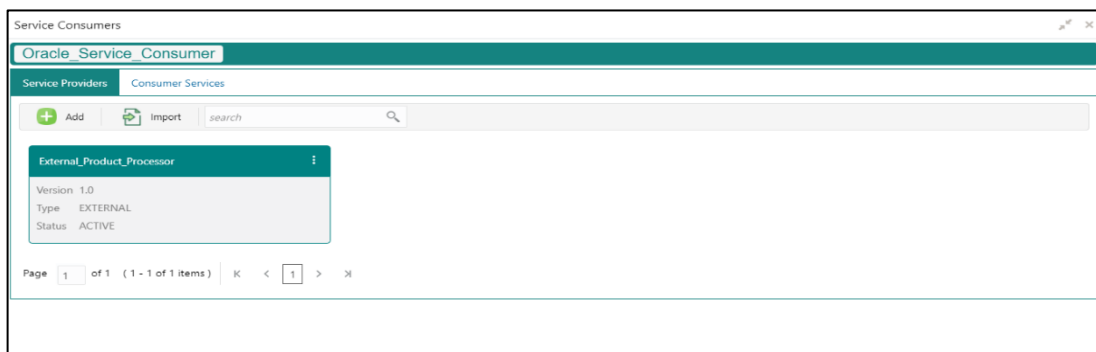
Figure 127: Service Providers
