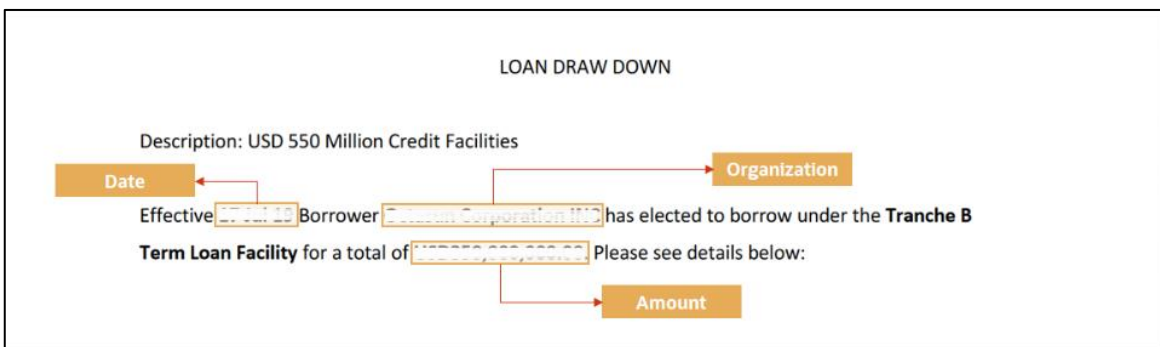
Figure 234: Annotator
