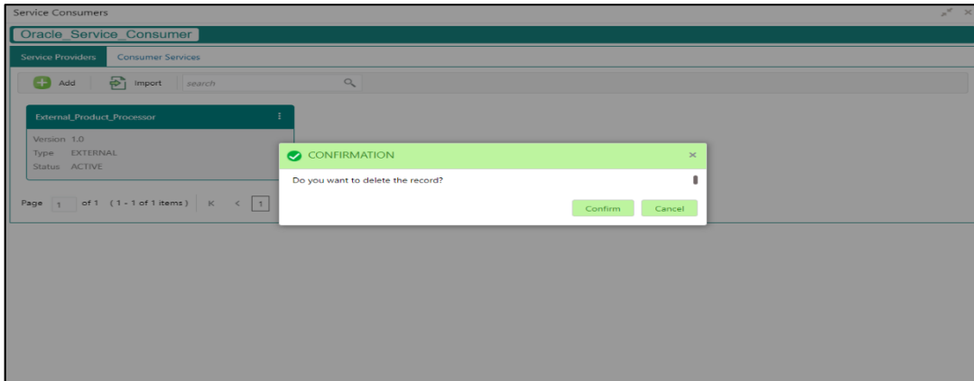
Figure 87: Delete
