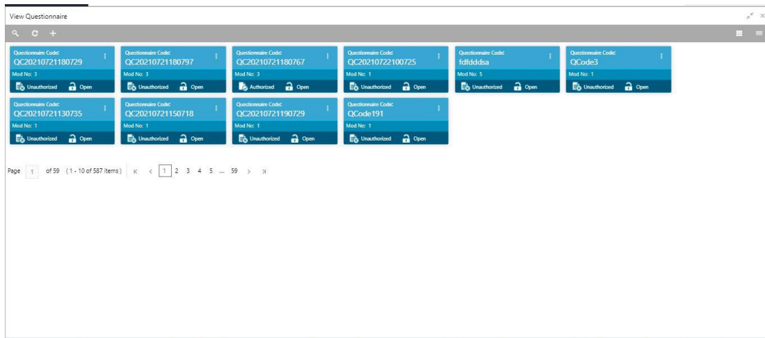
Figure 177 : View Questionnaire
