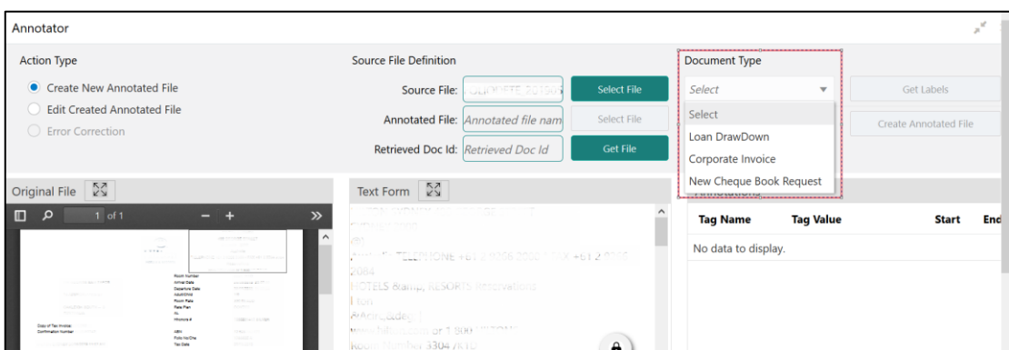
Figure 239: Document Type
