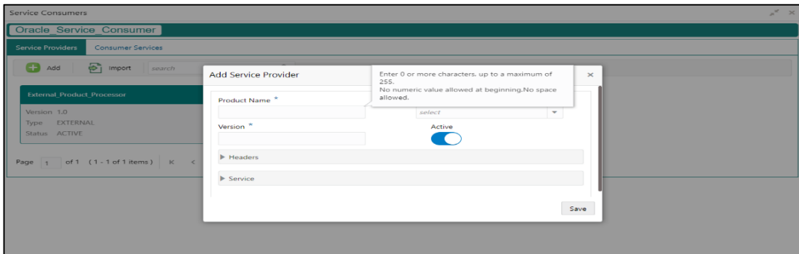
Figure 128: Add
