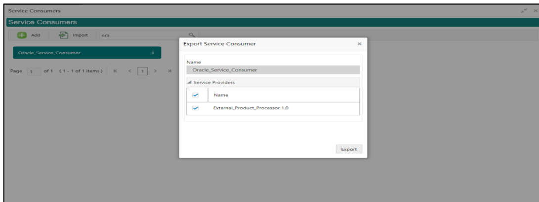
Figure 76: JSON Export
