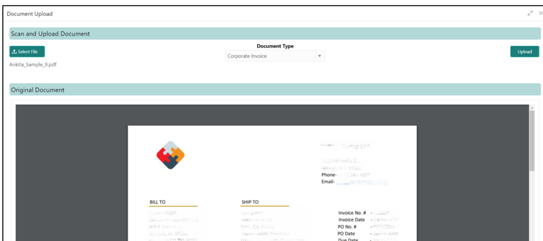
Figure 249: Document Upload
