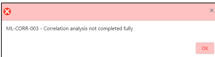
Figure 260: Error Message
