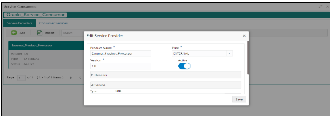
Figure 134: Edit
