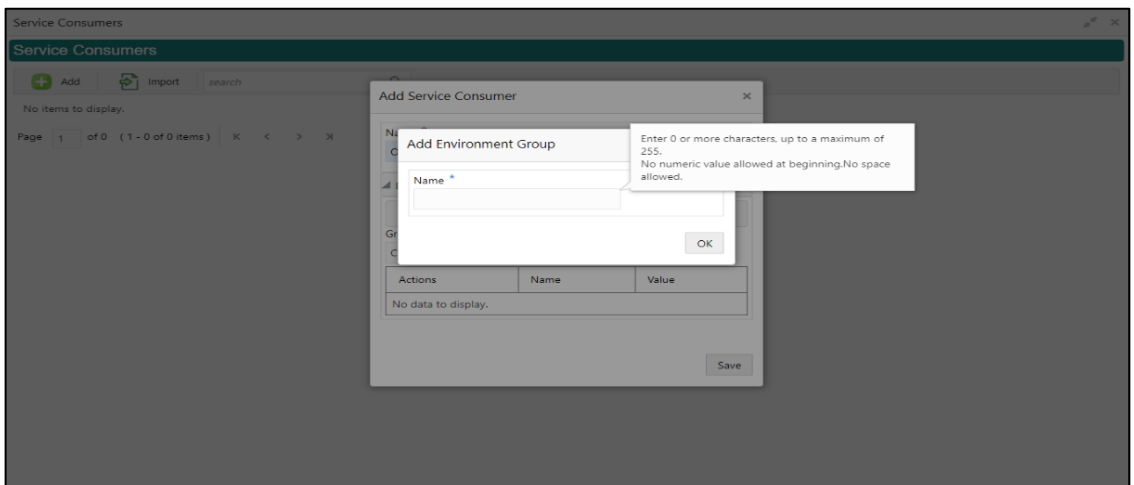
Figure 71: Environment Variables
