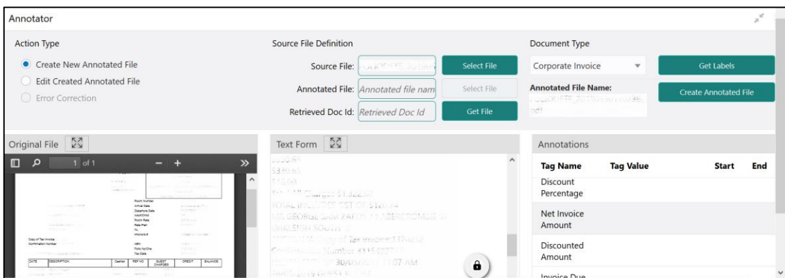
Figure 244: Tag Value
