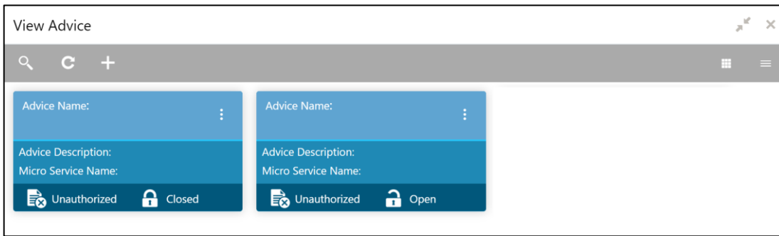
Figure 3: View Advice
